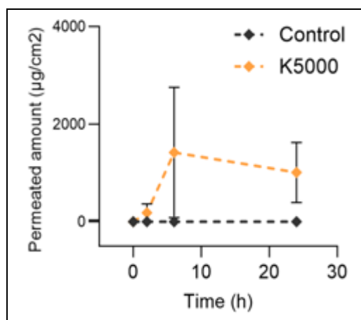
FIG. 3: TRANSDERMAL ABSORPTION OF SODIUM ASCORBATE CHANGE CURVE FOR CONTROL AND KERATINASE 5000 U MEASURED AT DIFFERENT TIME POINTS (DATA IS REPRESENTED AS A MEAN \pm SEM).
